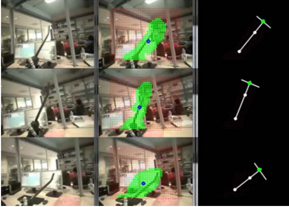
Figure 5: Explorative behavior for discovering the tool dimensions. Left: images acquired from the robot's camera; Middle: the output of the motionCUT module depicting the independent motion blobs; Right: extraction of the tool tip projection (green dot).
