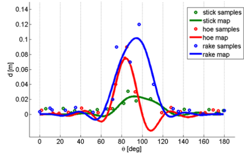
Figure 9: The maps retrieved for the pulling affordance with tools.
