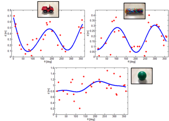
Figure 7: The maps of the rolling affordances for the toy car, the cylindrical tube and the small ball: red dots represent the sampled pairs of input angle \theta and the output distance d ; in blue the predictions provided by the learned maps M_{\text{roll}} over the whole input space.
