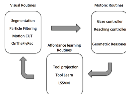
Figure 1: General overview of the iCub modules used in the experiments.
