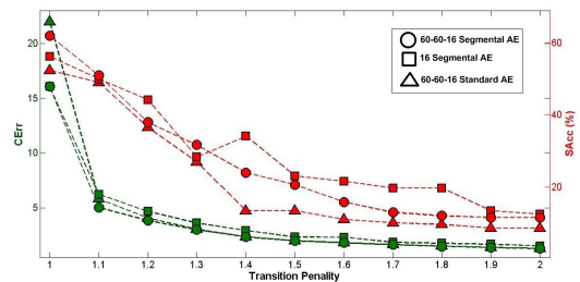
Fig. 1. Consistency error (green line) and word classification accuracy (red line) (in the Lecce dataset) of three systems as a function of the transition penalty value, the parameter affecting the expected dwell time.
