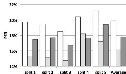
Figure 1: Phone Error Rate (PER) in each fold and on average for the cnz dataset using the following feature sets: MFSCs (white), MFSCs + actual AFs (light grey), MFSCs + recovered AFs (dark grey).
